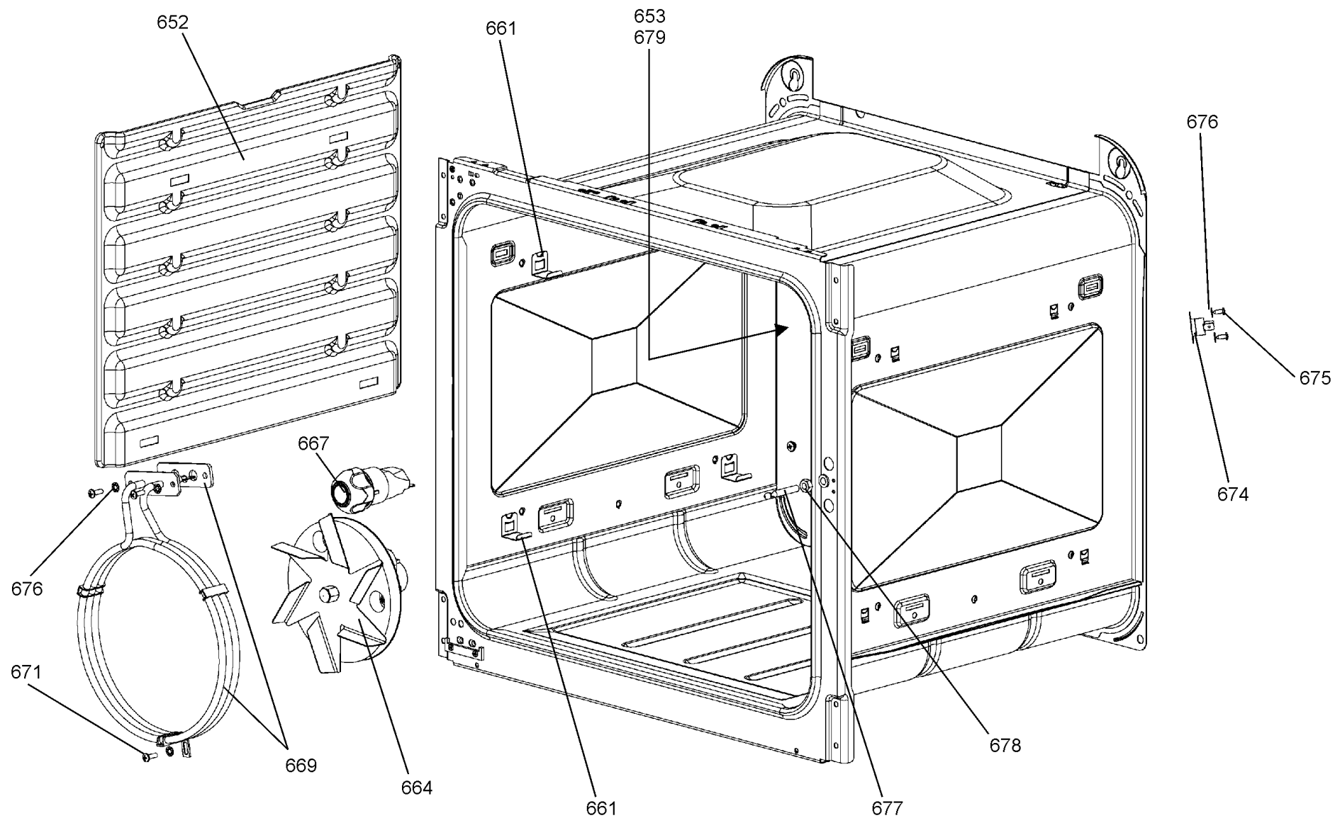
LH OVEN (FAN + LIGHT)
